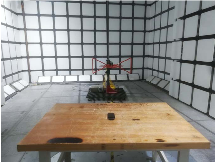
Radiated Spurious Emissions View (Below 1 GHz)
