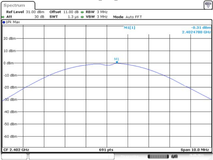
3DH1_Ant1_2402
