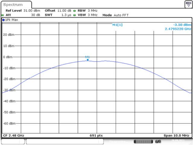
2DH1_Ant1_2480
