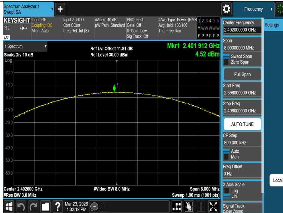
3DH5-Ant1-2402-PASS
