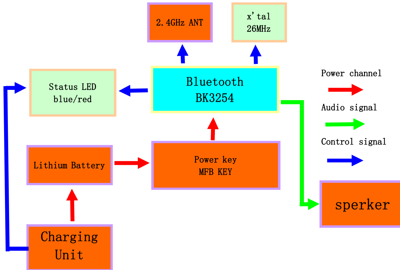
HP0363-BK3254 Block Diagram
