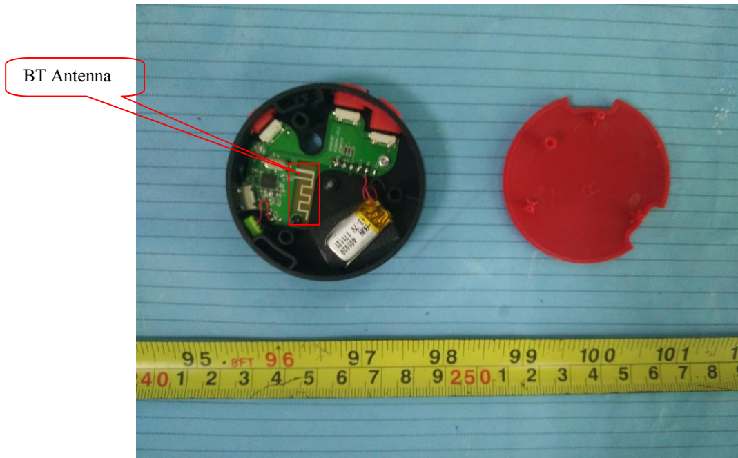
EUT – Cover off View 6
