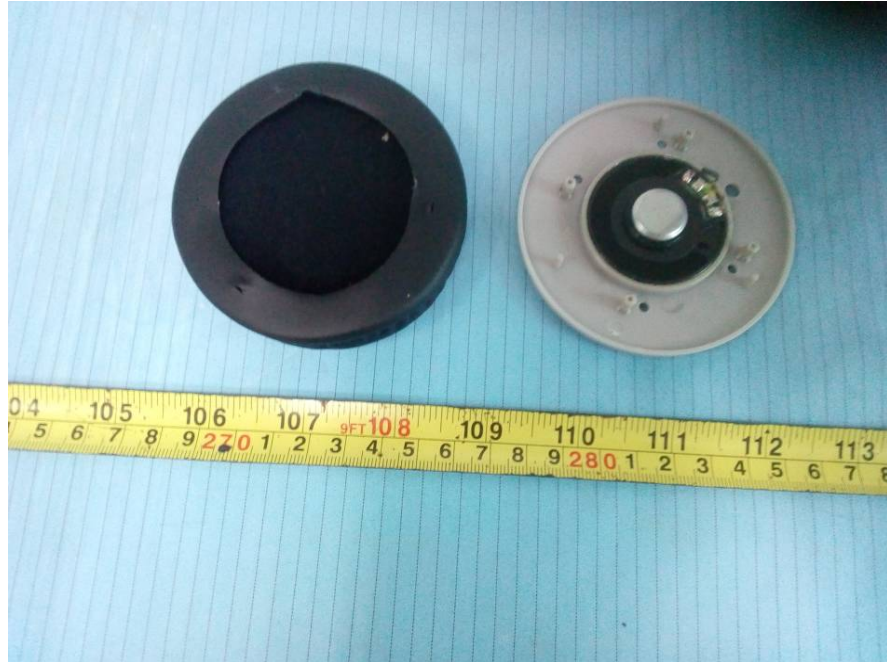
EUT – Cover off View 3 (Left Ear)
