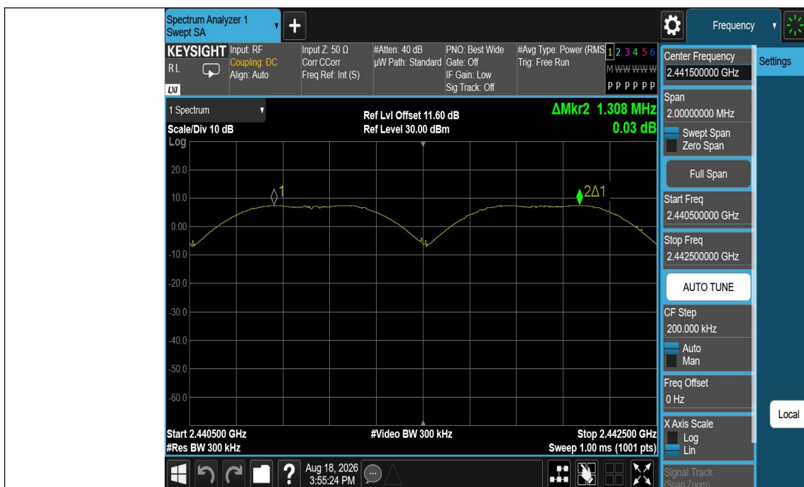
DH5-Ant1-Hop-PASS
