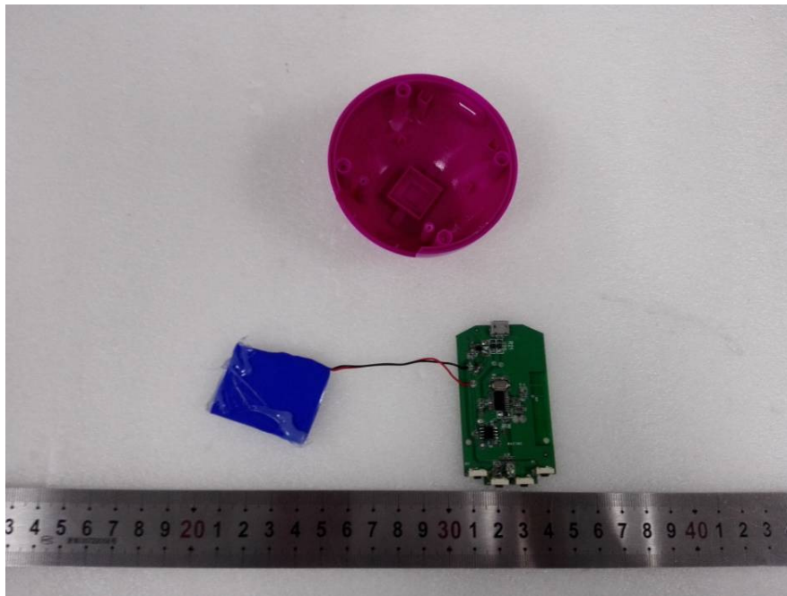
EUT 1 – Cover off View 3
