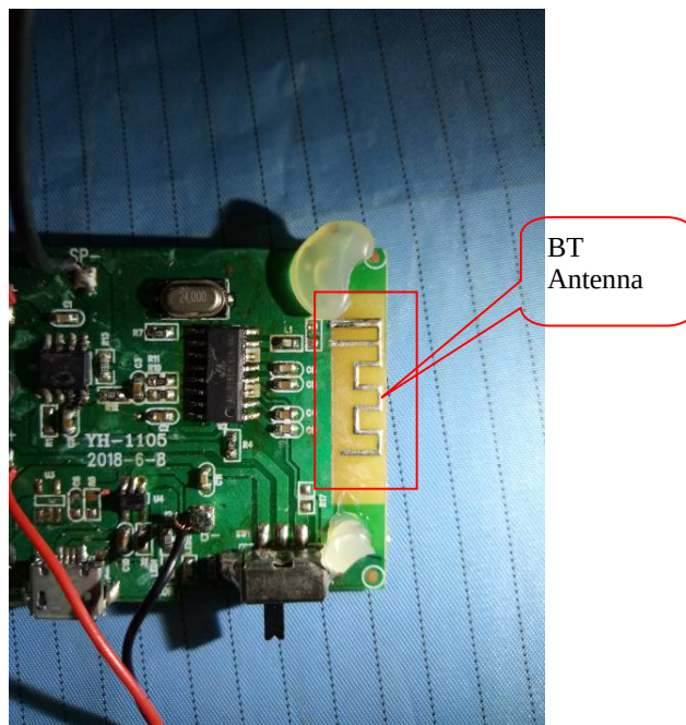
EUT – Main IC View 1
