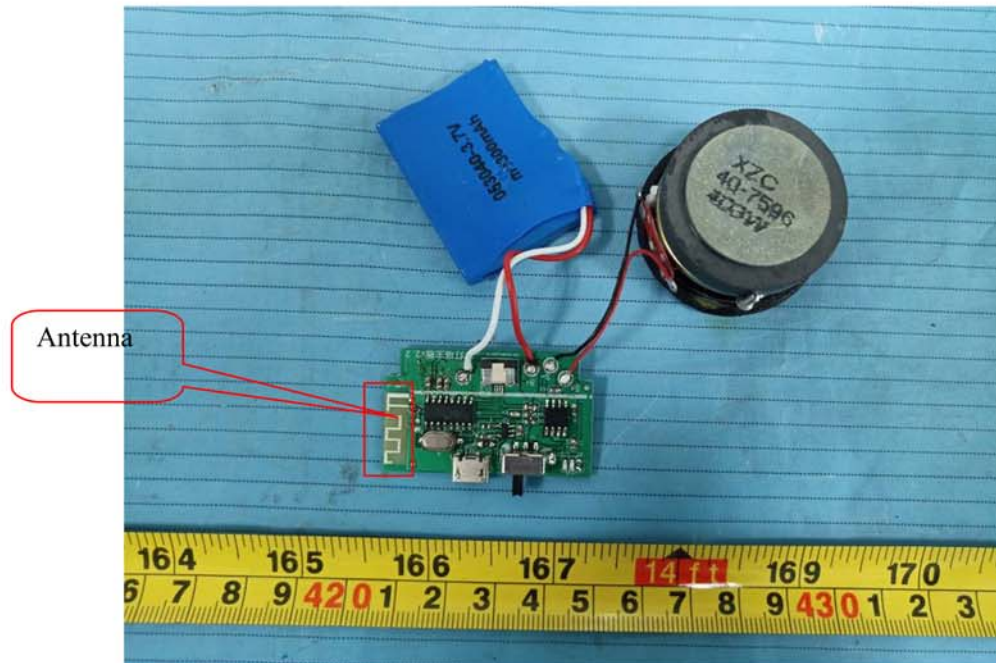
EUT – Main Board&Battery Top View
