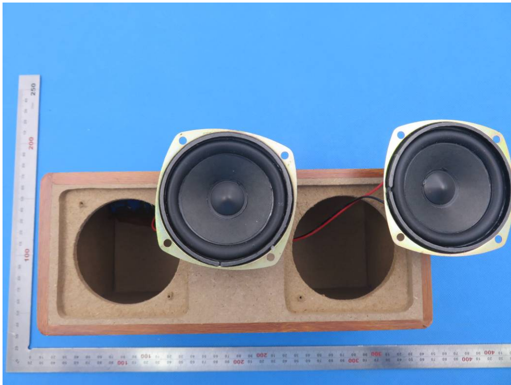
OPEN VIEW OF EUT-2 (SP-0272)
