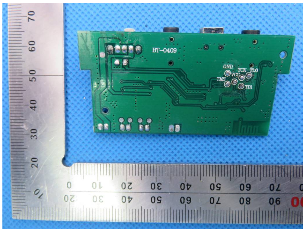
INTERNAL VIEW OF EUT-2 (SP-0272)
