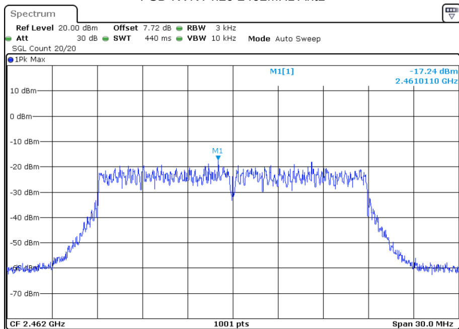
PSD NVNT n20 2462MHz Ant1
