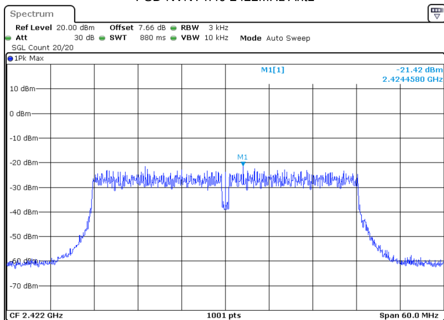
PSD NVNT n40 2422MHz Ant1
