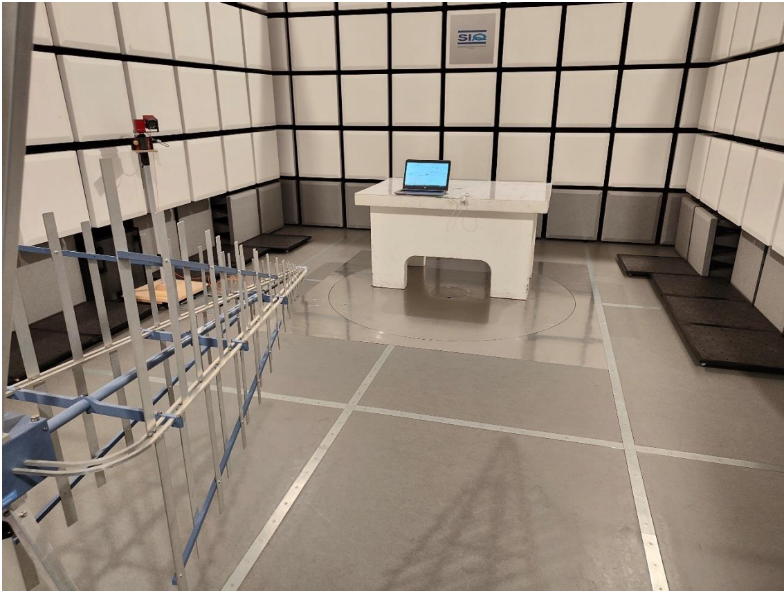
Figure 2: Radiated emission test till 1 GHz
