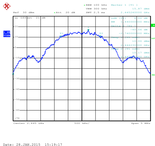
Figure 8.2-1: 6 dB bandwidth sample
