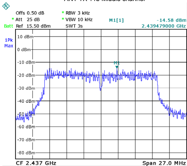
ANT TX 11b Middle channel
