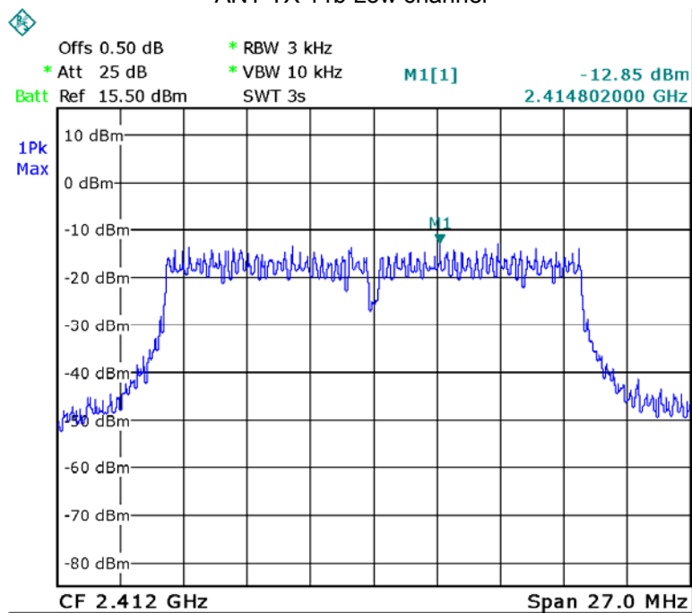
ANT TX 11b Low channel
