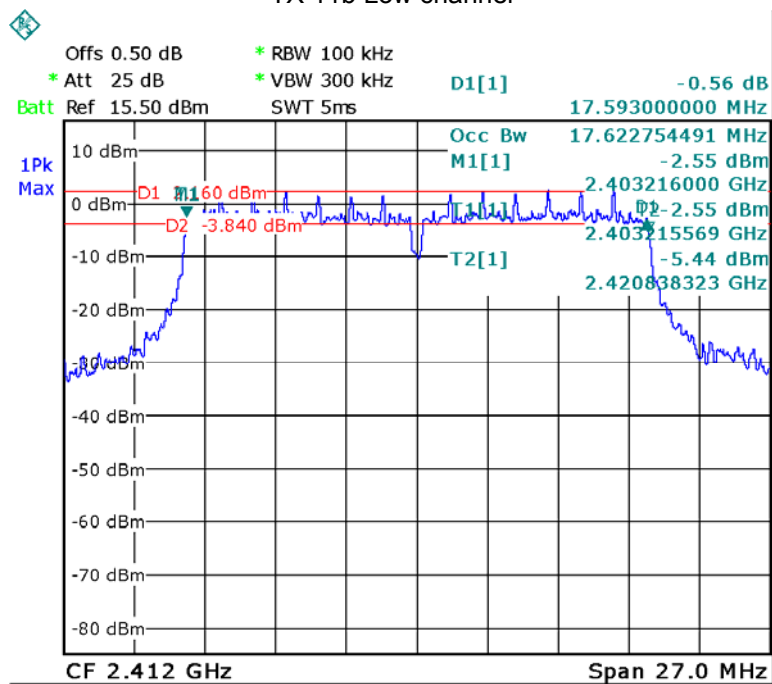
TX 11b Low channel
