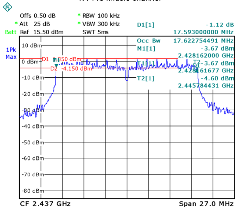
TX 11b Middle channel
