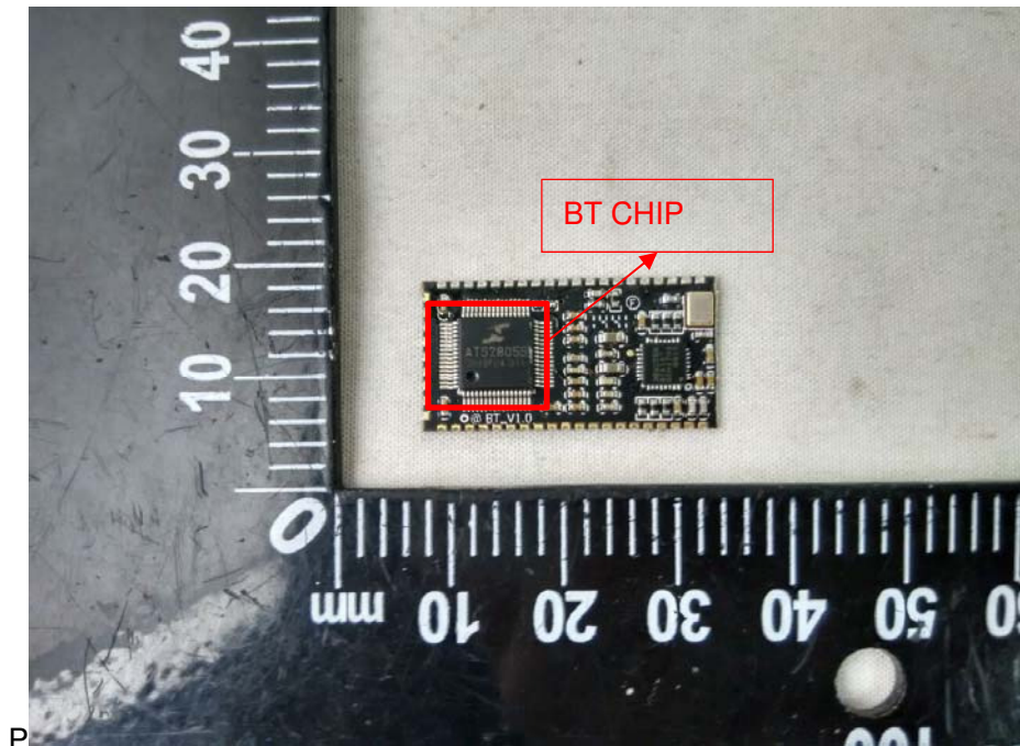
MAIN BOARD TOP VIEW 2
