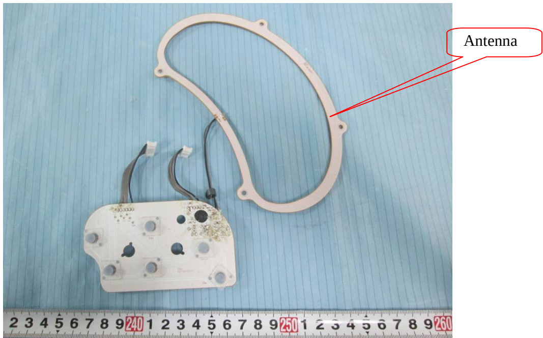
EUT – Keyboard Top View
