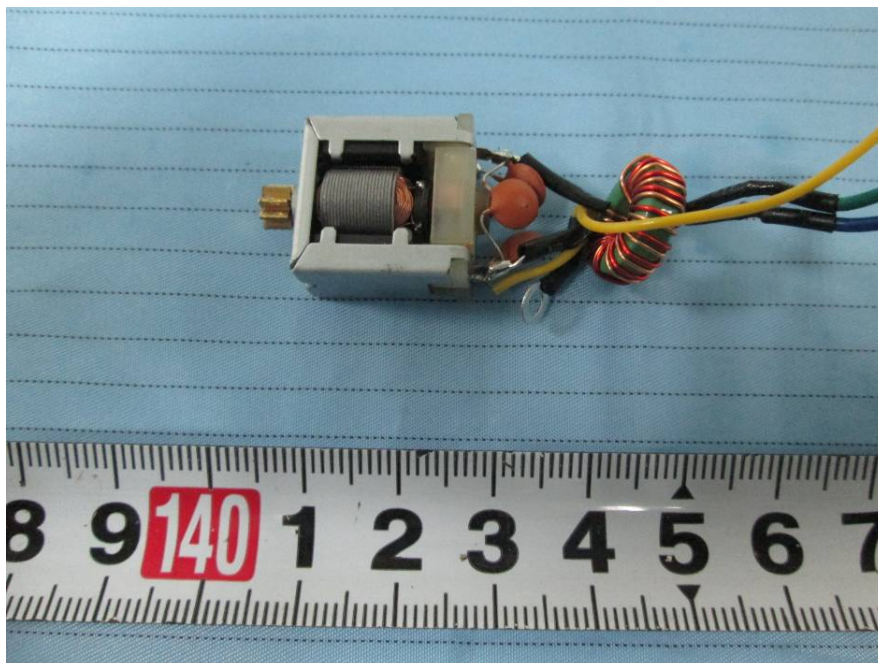
EUT – MotorView
