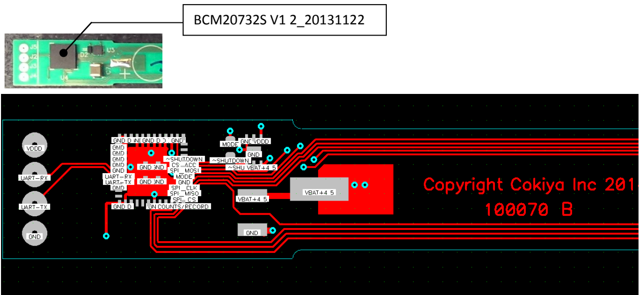
Top layer artwork
