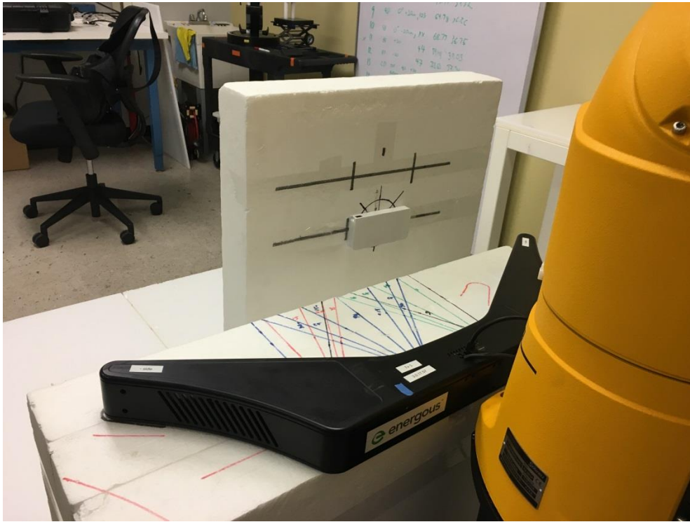
Client device at 30^\circ , 50 cm from the MS-300. Other angular offsets follow a similar setup.
