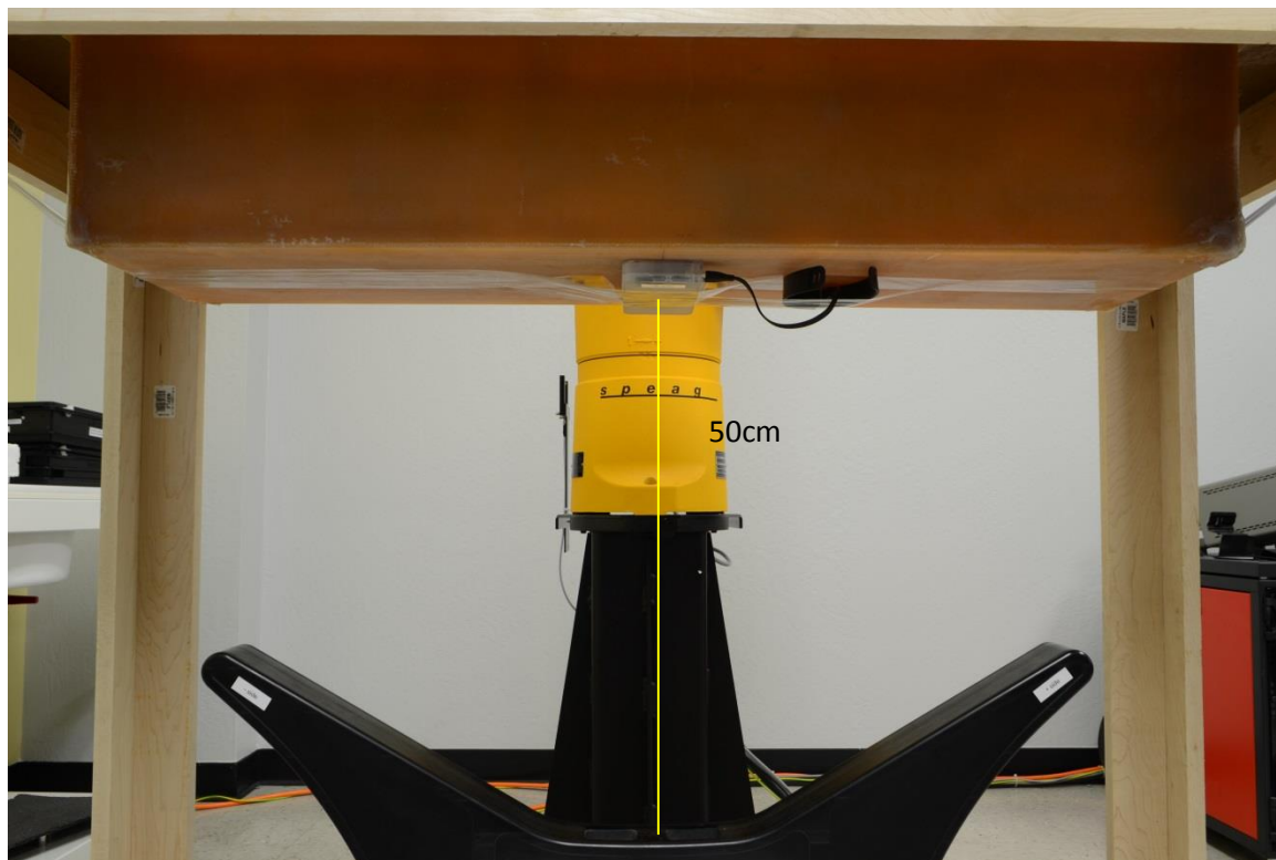
DUT located under Phantom (0 degrees, 50cm with watch connected to client device)
