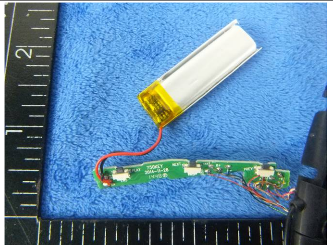
Small Board & Battery - Front View
