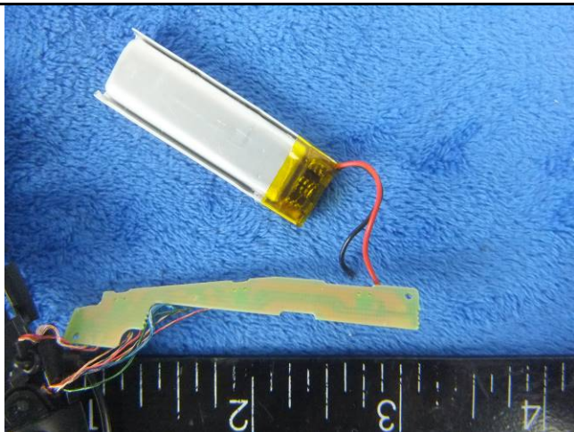
Small Board & Battery - Rear View
