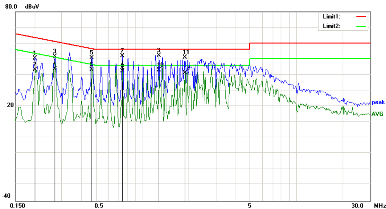
Phase Natural Plot at 240V AC, 60Hz
