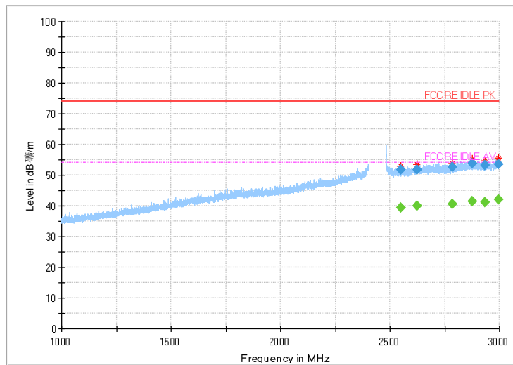
Fig.49 Radiated Spurious Emission (802.11b,Ch12,1GHz~3GHz)
