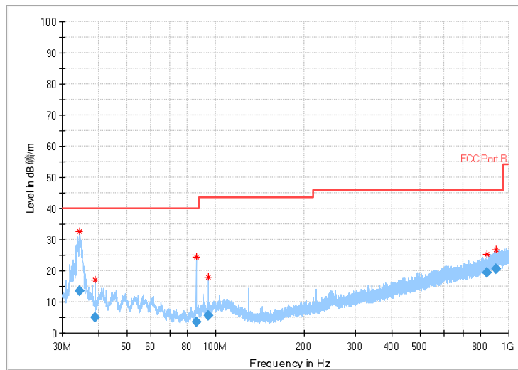
Fig.51 Radiated Spurious Emission (802.11g, Ch13, 30MHz~1GHz)
