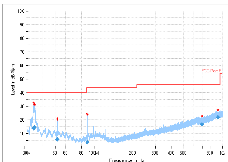
Fig.48 Radiated Spurious Emission (802.11n,Ch12,30MHz~1GHz)
