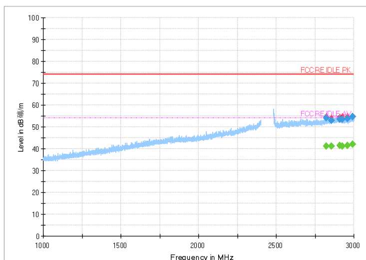
Fig.49 Radiated Spurious Emission (802.11g,Ch12,1GHz~3GHz)
