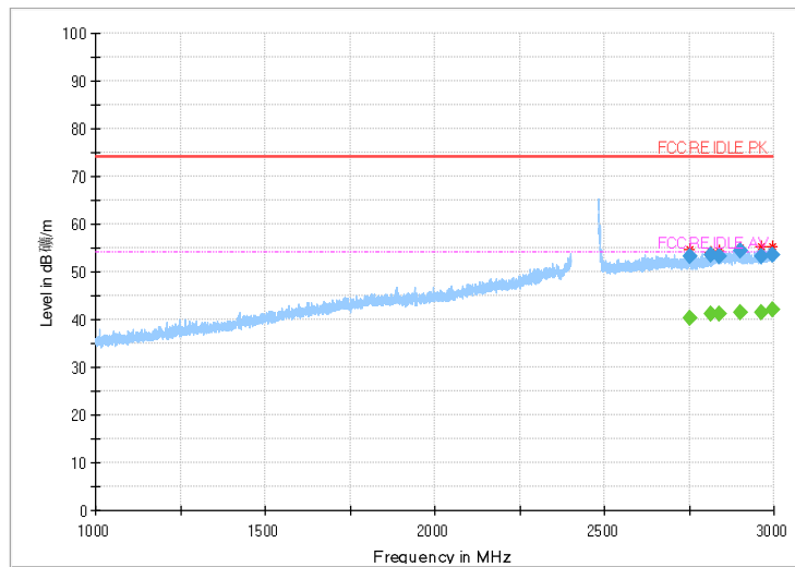
Fig.52 Radiated Spurious Emission (802.11n,Ch13,1GHz~3GHz)
