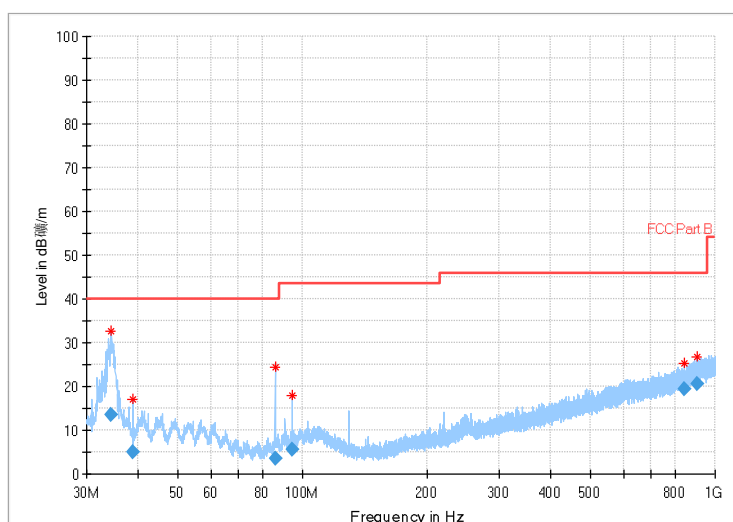
Fig.51 Radiated Spurious Emission (802.11b,Ch13,30MHz~1GHz)
