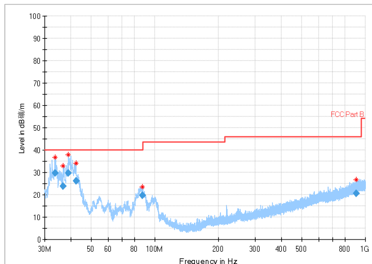
Fig.51 Radiated Spurious Emission (802.11n,Ch13,30MHz~1GHz)
