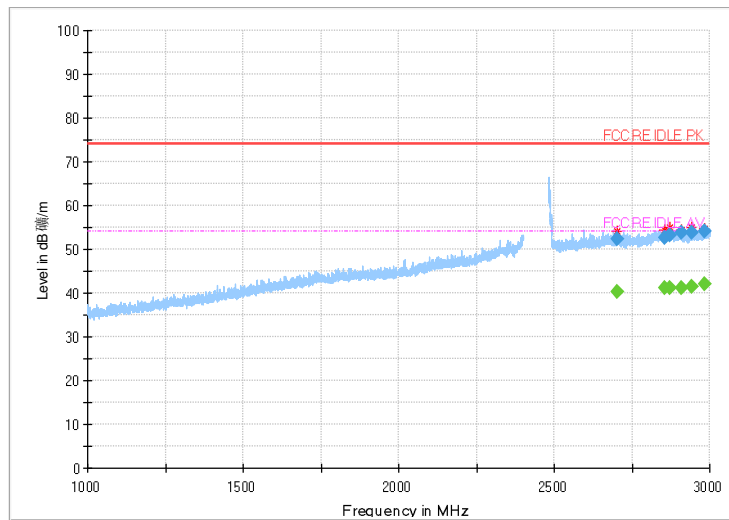
Fig.52 Radiated Spurious Emission (802.11b,Ch13,1GHz~3GHz)
