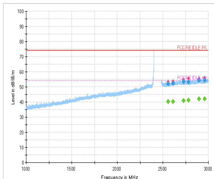
Fig.51 Radiated Spurious Emission (802.11g, Ch1, 1GHz~3GHz)
