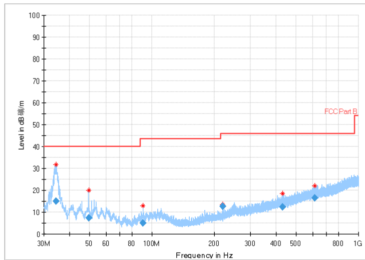
Fig.48 Radiated Spurious Emission (802.11b,Ch12,30MHz~1GHz)
