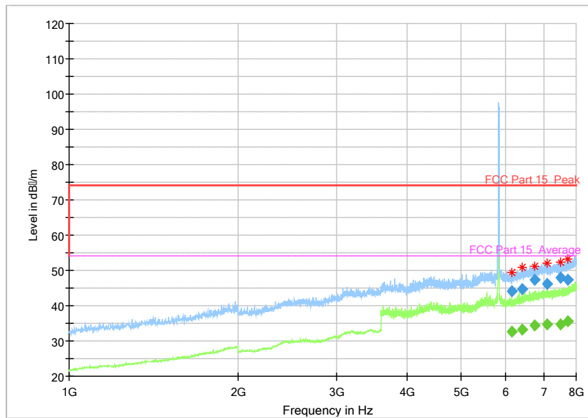
Fig. 30 Radiated emission: 802.11n, (802.11a, Ch165, 1 GHz - 8 GHz)
