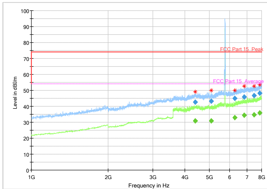
Fig. 44 Radiated Spurious Emission (802.11a, Ch149, 1 GHz-8 GHz)
