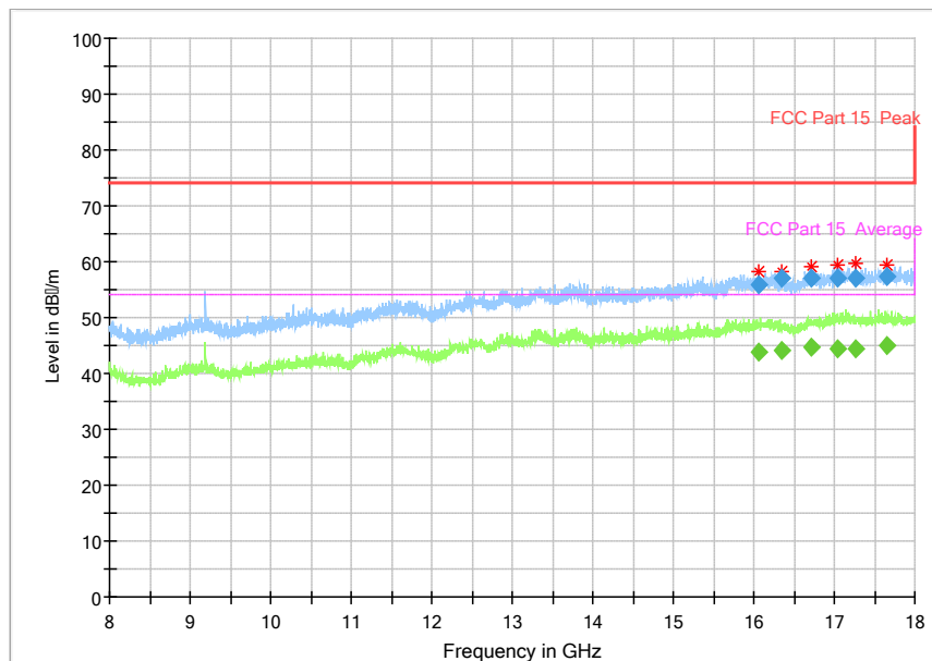
Fig. 45 Radiated Spurious Emission (802.11a, Ch149, 8 GHz-18 GHz)
