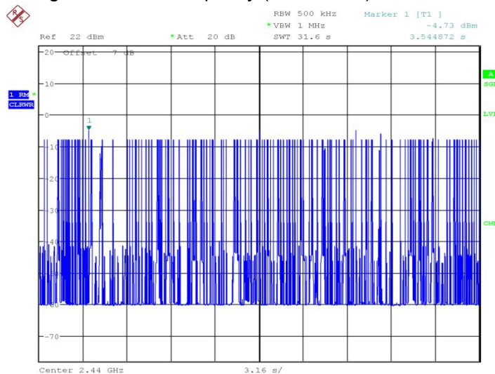
Fig.47 Time of occupancy (Dwell Time): Ch39, Packet DH3
