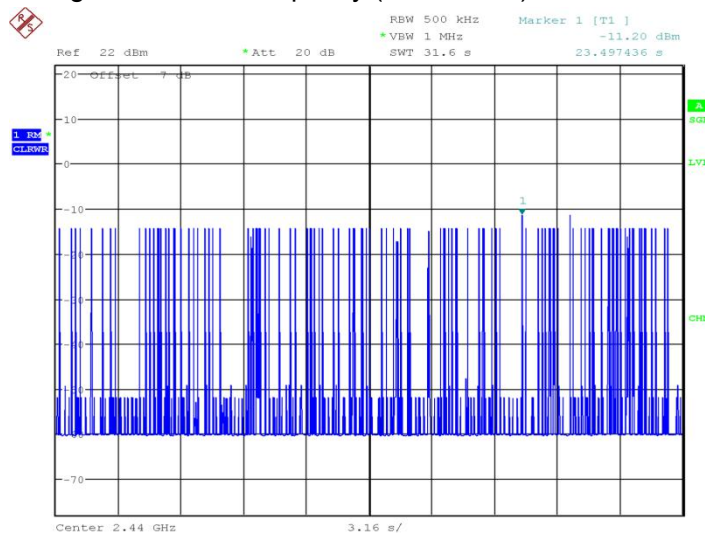
Fig.45 Time of occupancy (Dwell Time): Ch39, Packet DH1
