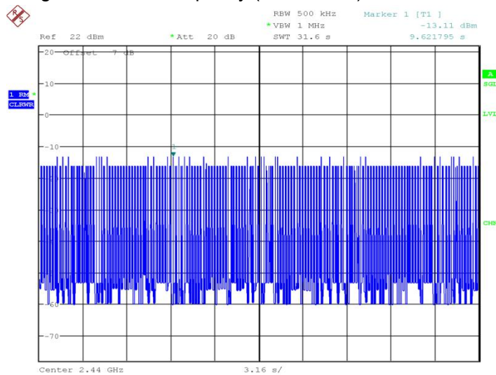
Fig.51 Time of occupancy (Dwell Time): Ch39, Packet 2-DH1
