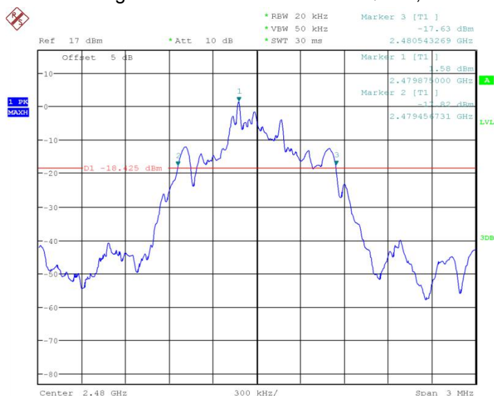
Fig.67 20dB Bandwidth: \pi/4 DQPSK, Ch39
