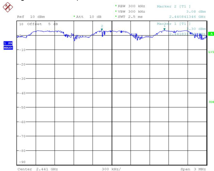
Fig.73 Carrier separation measurement: \pi/4 DQPSK, Ch39
