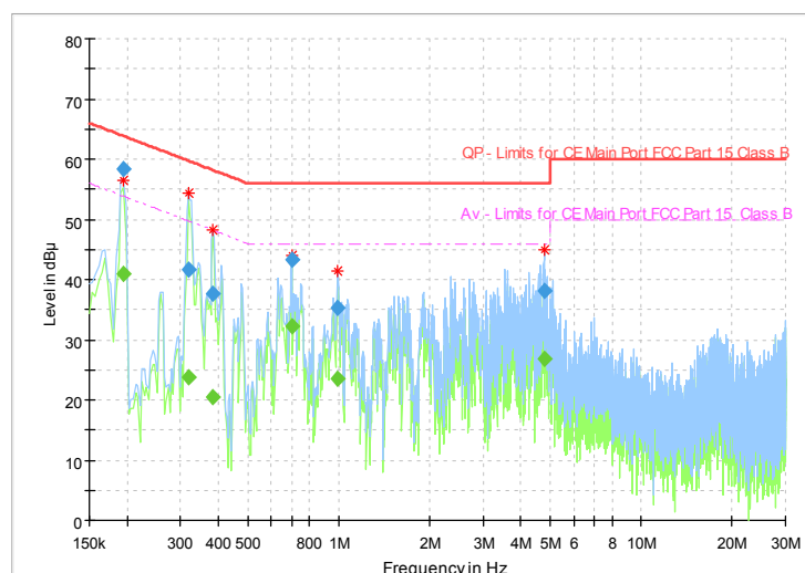
Fig.81 AC Powerline Conducted Emission
