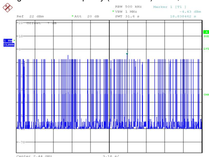
Fig.55 Time of occupancy (Dwell Time): Ch39, Packet 2-DH5
