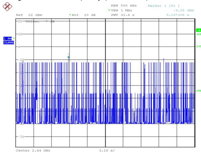
Fig.61 Time of occupancy (Dwell Time): Ch39,Packet 3-DH5
