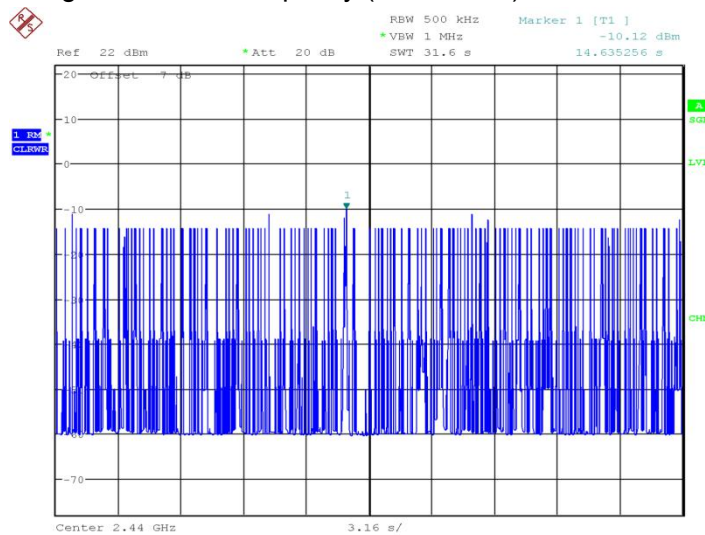
Fig.59 Time of occupancy (Dwell Time): Ch39,Packet 3-DH3
