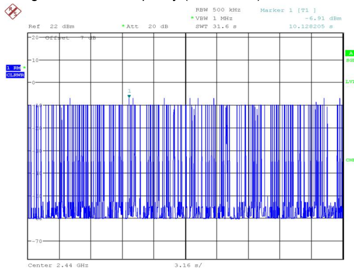
Fig.53 Time of occupancy (Dwell Time): Ch39,Packet 2-DH3
