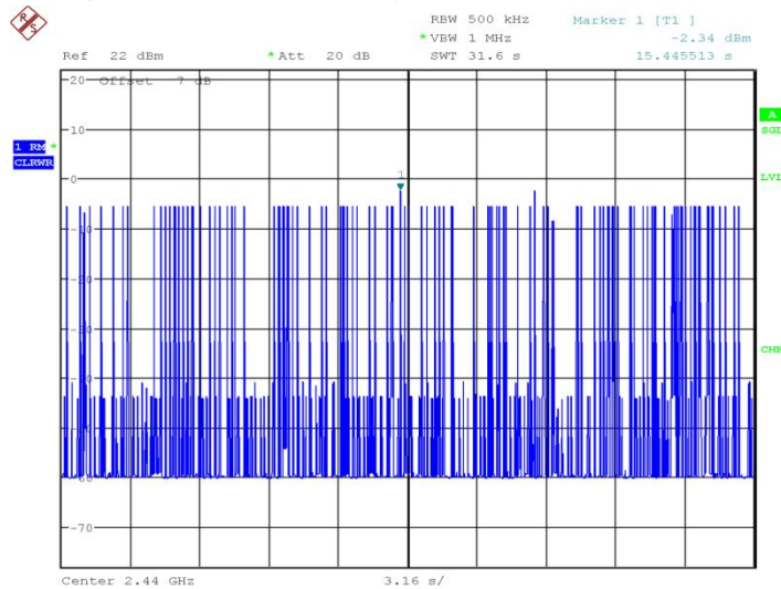
Fig.49 Time of occupancy (Dwell Time): Ch39,Packet DH5
