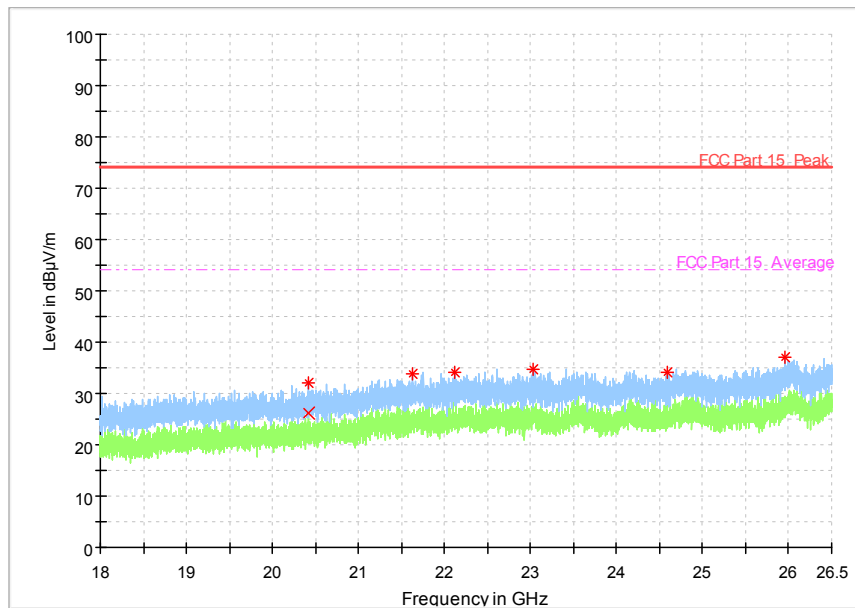
Fig. 36 Radiated Spurious Emission (802.11n-HT20, Ch149, 18 GHz-26.5 GHz)
