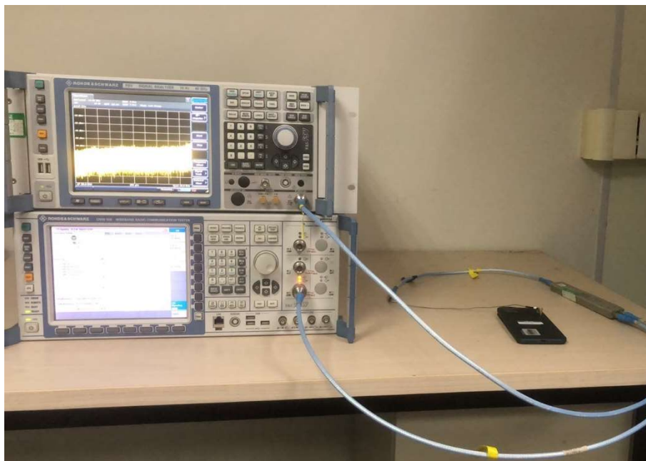
RF Conducted Test
