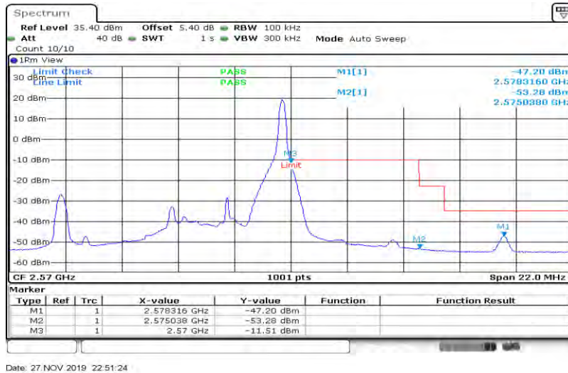
Band7-5MHz-16QAM-21425-25RB#0
