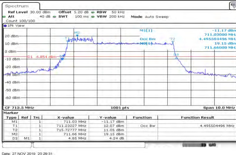
Band12-10MHz-QPSK-23060-50RB#0-8.971
