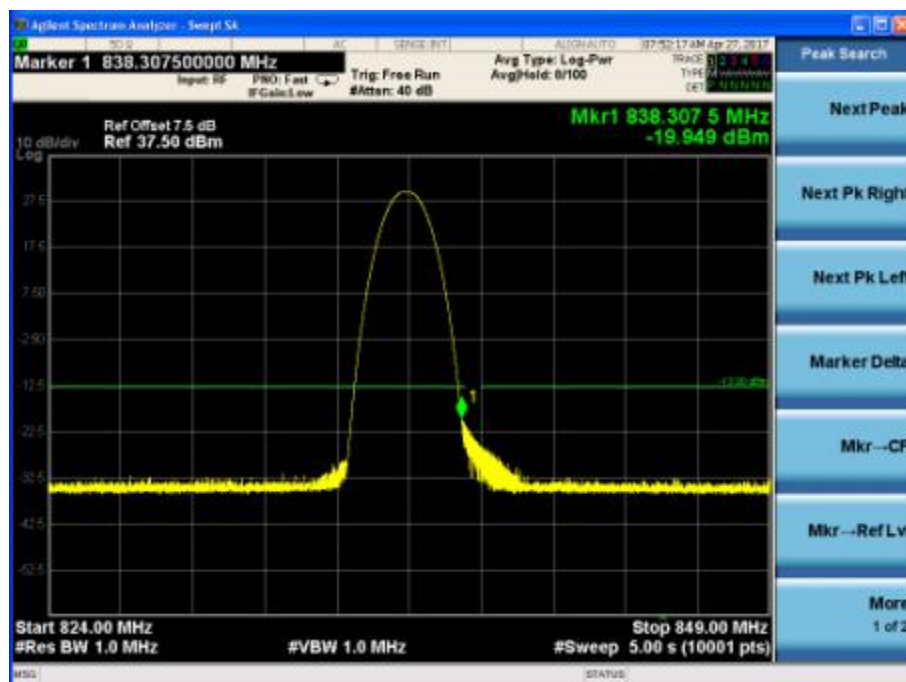
Channel 189, 824MHz~849MHz
