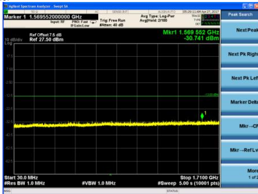
Channel 1412, 30MHz~1710MHz
