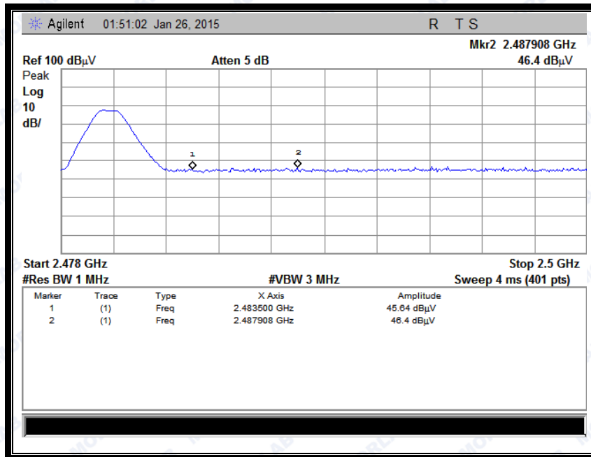
(Plot B1: Channel = 39 PEAK)
