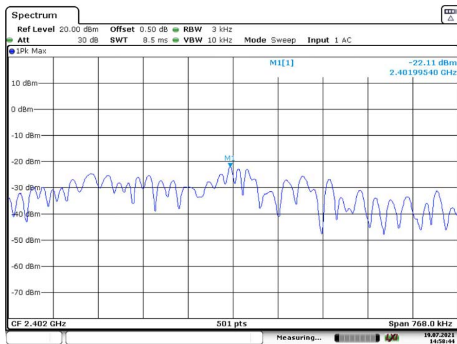
Power Spectral Density, 1Mbps, Low Channel
