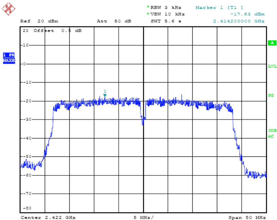
Channel 03 (2422MHz)
