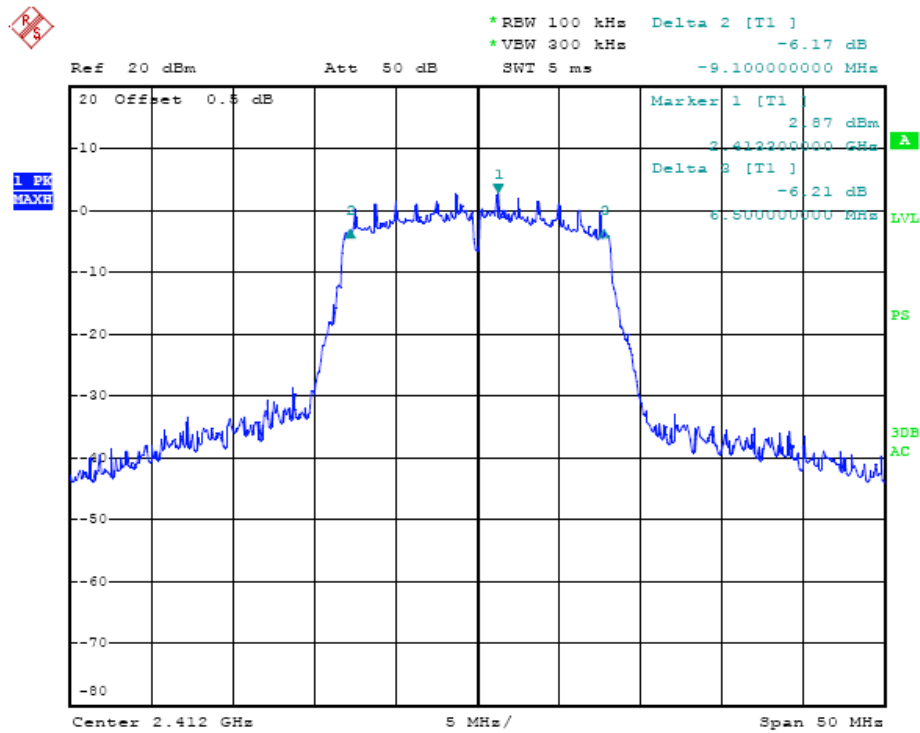
Channel 01 (2412MHz)
