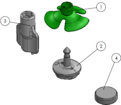
Figure 20: Battery exchange set
