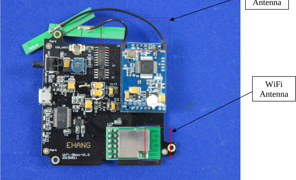
Figure 9 PCB of the EUT-Front View
