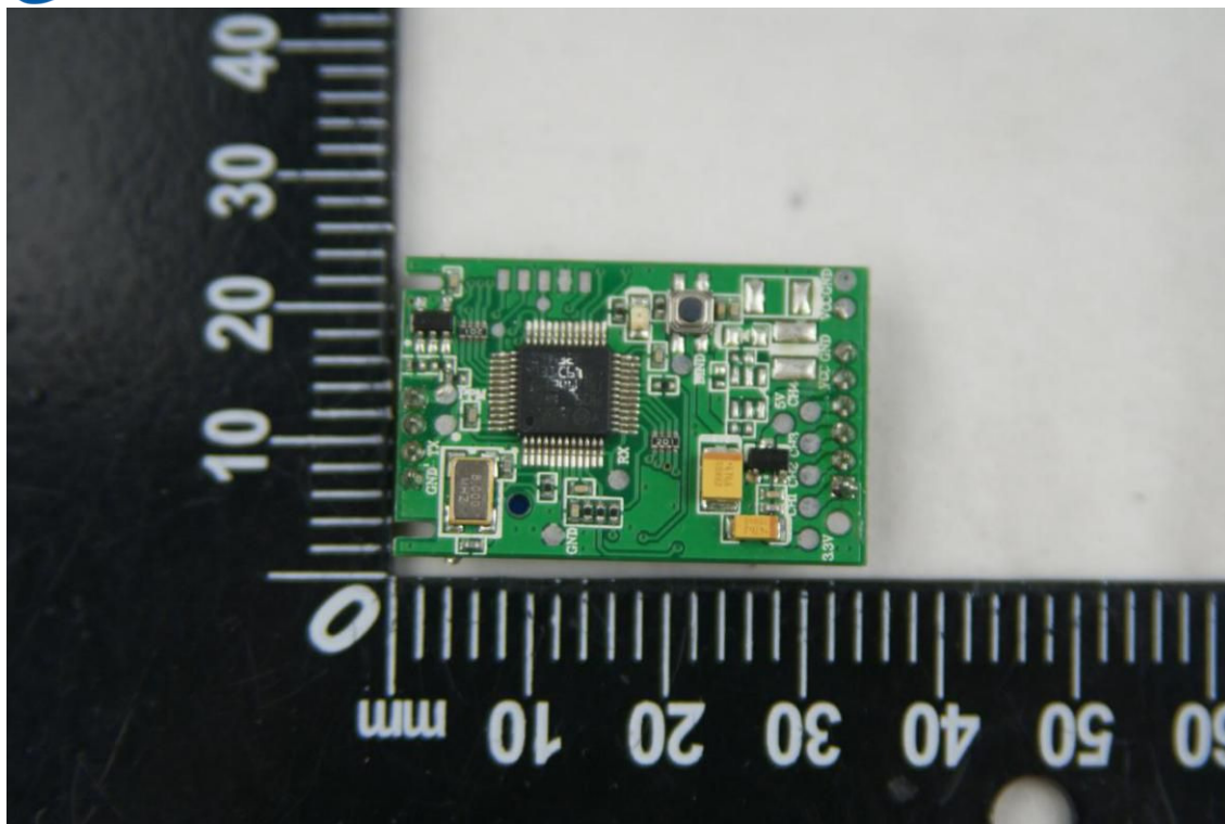
EUT PHOTO 29(2.4G model)
