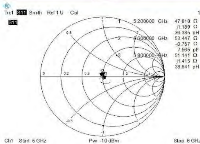
Impedance
