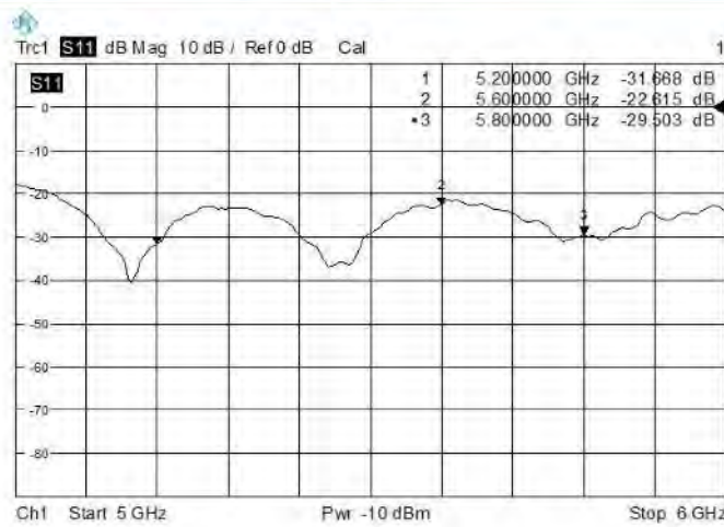
Return Loss
