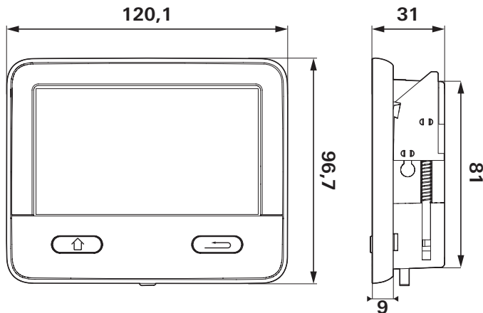
Figure 2 – Dimensions in mm. Illustration not to scale
