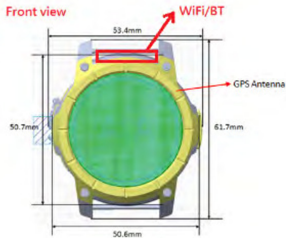
Antenna location (front view)
