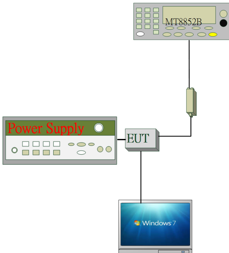
Fig. 2-2 Conducted (Antenna Port)
