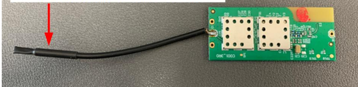
FHSS Antenna (Tx and Rx) 903.28 MHz - 925.36 MHz
