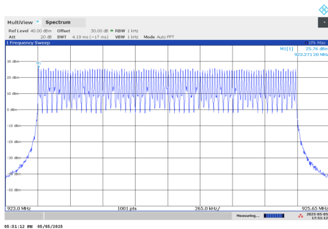
Figure 7.4-7: Number of hopping channels
