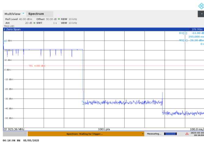
Figure 7.4-9: Dwell time, in sweep time 1s
