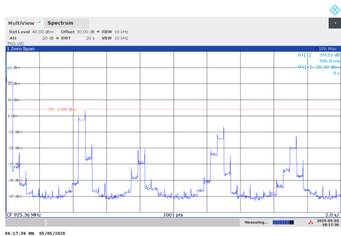
Figure 7.4-10: Dwell time, in sweep time 20s
