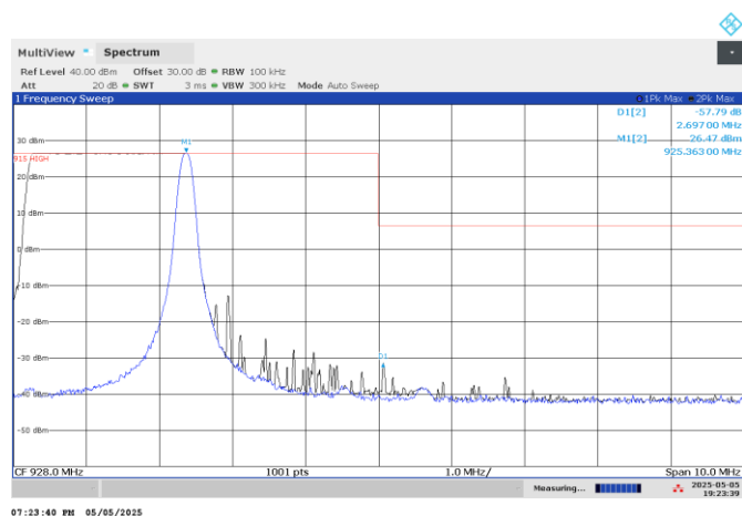
Figure 7.6-4: Band edge spurious emissions, Hopping on highest frequency group
