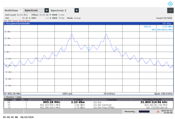
Figure 7.4-4: 99% occupied bandwidth on low channel
