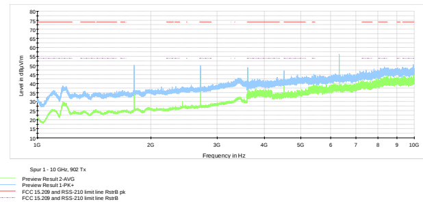
Figure 7.6-11: Radiated spurious emissions on above 1 GHz, Low ch.
