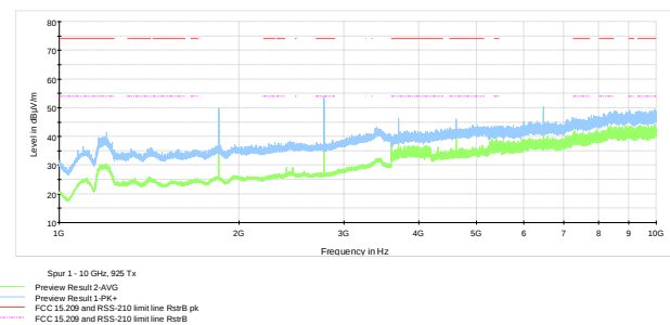
Figure 7.6-13: Radiated spurious emissions on above 1 GHz, High ch.
