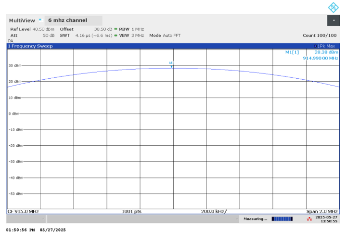
Figure 7.5-2: Output power on mid channel
