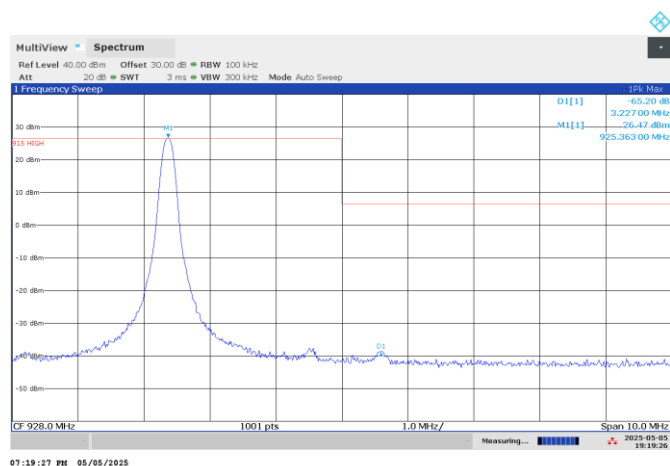
Figure 7.6-2: Band edge spurious emissions at 925.36 MHz
