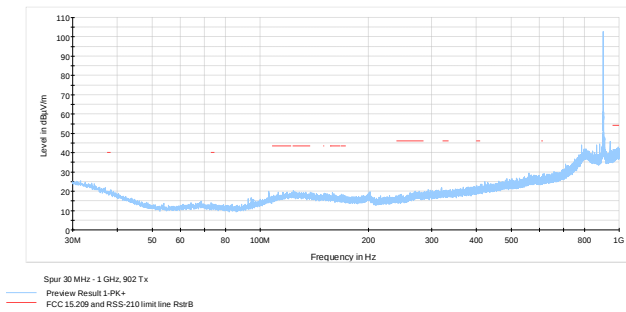
Figure 7.6-8: Radiated spurious emissions on below 1 GHz, Low ch.
