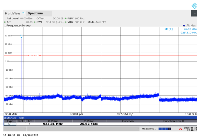
Figure 7.6-7: Conducted spurious emissions at high ch
