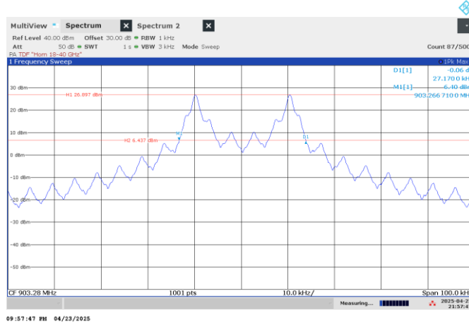
Figure 7.4-1: 20 dB bandwidth on low channel
