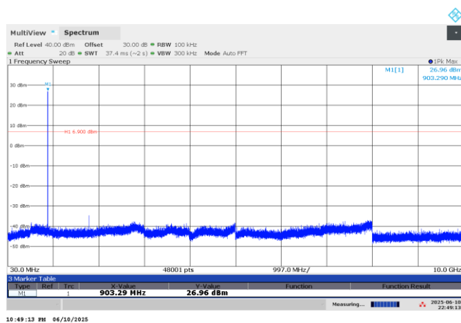
Figure 7.6-5: Conducted spurious emissions at low ch
