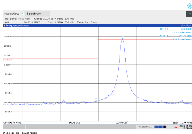
Figure 7.6-1: Band edge spurious emissions at 903.28 MHz
