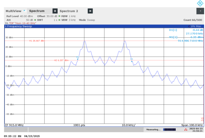
Figure 7.4-2: 20 dB bandwidth on mid channel
