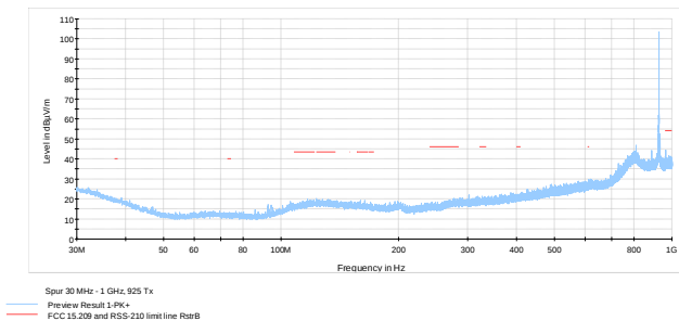
Figure 7.6-10: Radiated spurious emissions on below 1 GHz, High ch.
