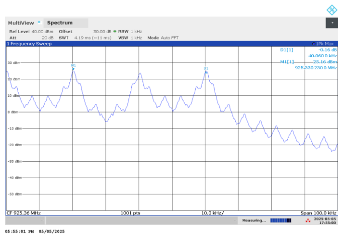
Figure 7.4-8: Carrier frequency separation
