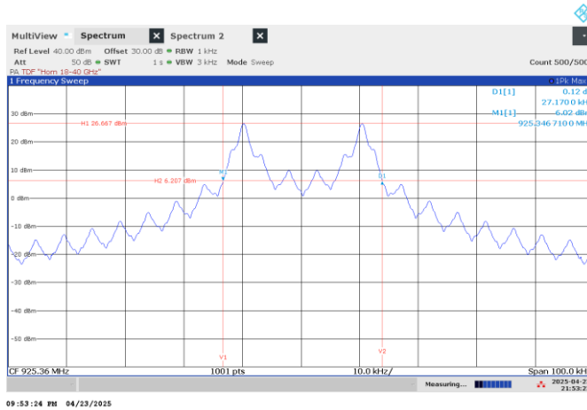
Figure 7.4-3: 20 dB bandwidth on high channel
