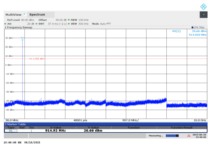
Figure 7.6-6: Conducted spurious emissions at mid ch
