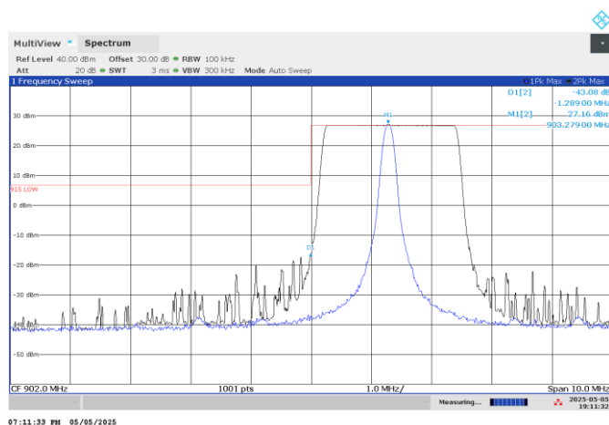
Figure 7.6-3: Band edge spurious emissions, Hopping on lowest frequency group
