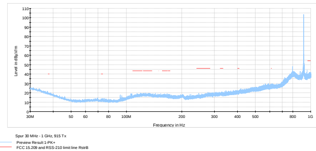
Figure 7.6-9: Radiated spurious emissions on below 1 GHz, Mid ch.
