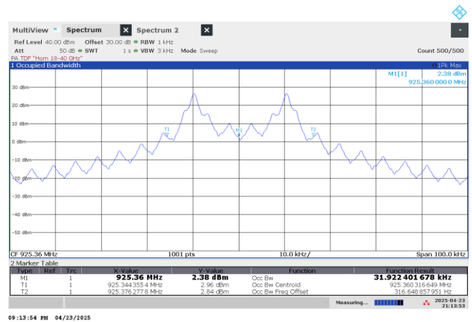
Figure 7.4-6: 99% occupied bandwidth on high channel
