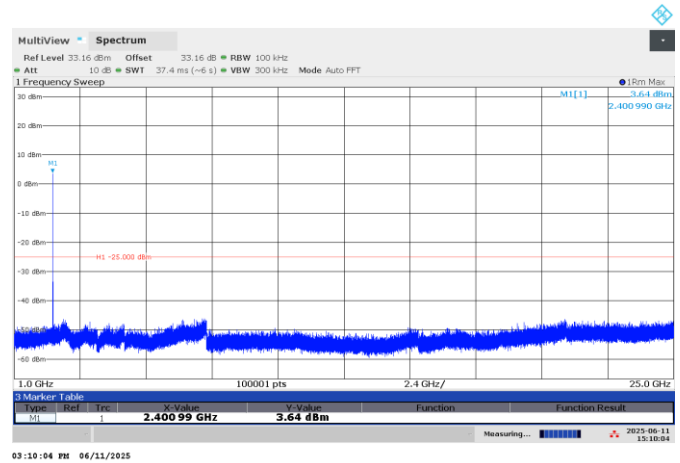
Figure 7.6-8: Conducted spurious emissions on above 1 GHz, Low ch.
