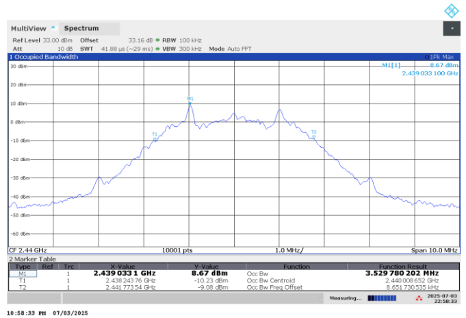
Figure 7.4-5: 99% occupied bandwidth on GFSK, Mid ch
