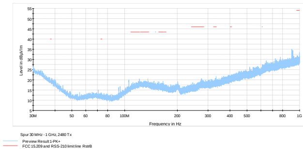
Figure 7.6-13: Radiated spurious emissions on below 1 GHz, High ch.
