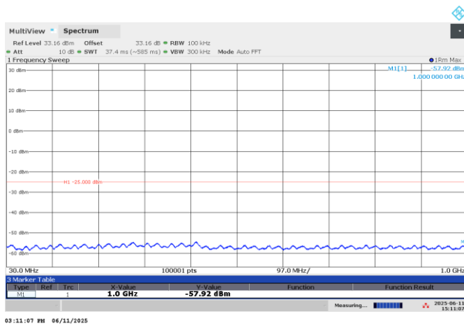
Figure 7.6-5: Conducted spurious emissions on below 1 GHz, Low ch.
