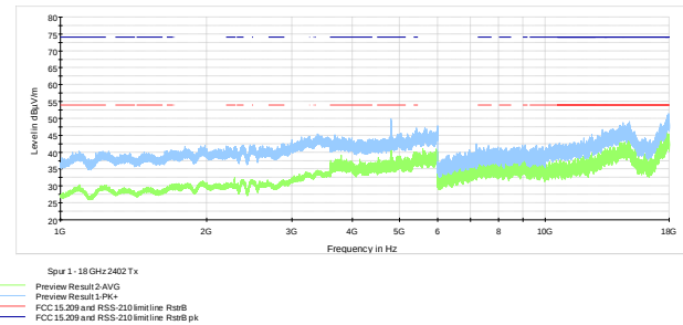
Figure 7.6-14: Radiated spurious emissions on 1 - 18 GHz, Low ch.
