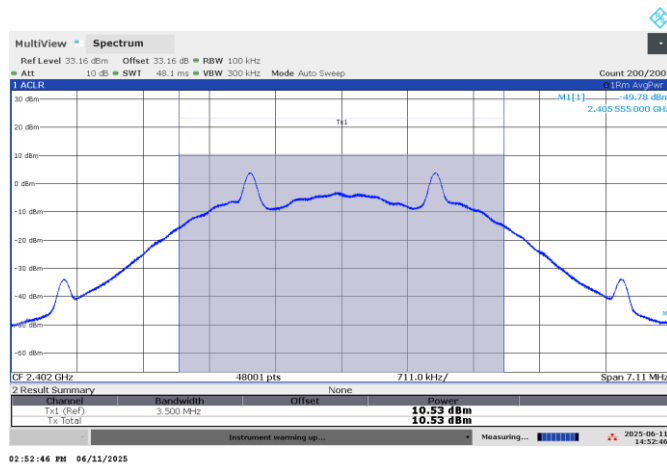
Figure 7.5-1: Output power on low channel
