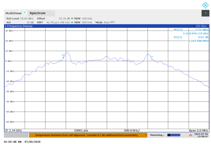
Figure 7.4-2: 6 dB bandwidth GFSK, Mid ch.
