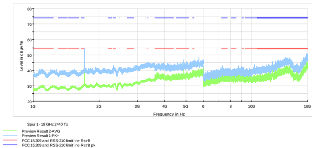
Figure 7.6-15: Radiated spurious emissions on 1 - 18 GHz, Mid ch.
