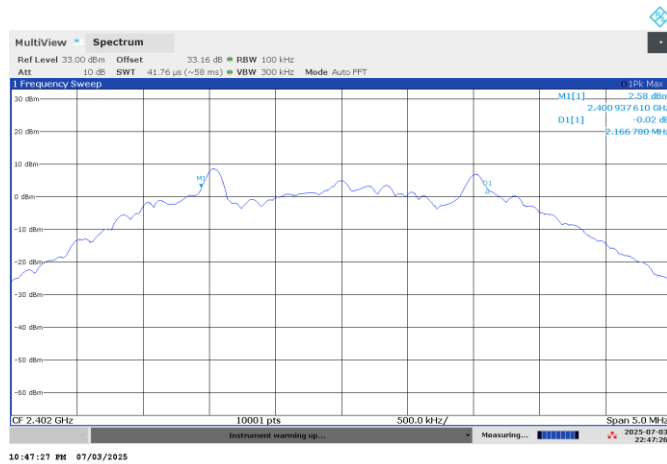
Figure 7.4-1: 6 dB bandwidth on GFSK, Low ch.
