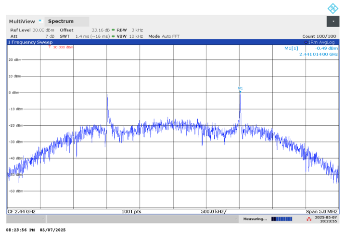
Figure 7.7-2: PSD on mid channel
