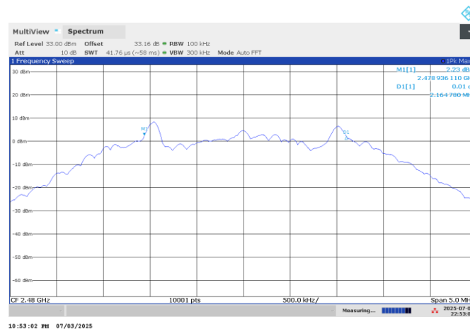
Figure 7.4-3: 6 dB bandwidth on GFSK, High ch.
