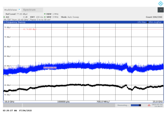
Figure 7.6-18: Radiated spurious emissions on 18 -25 GHz, Mid ch.
