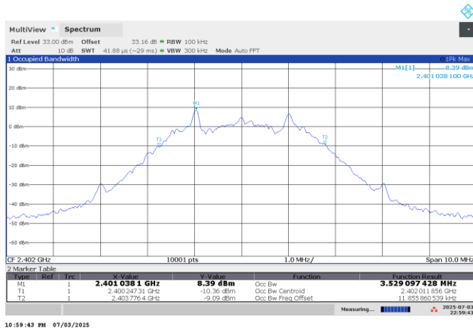
Figure 7.4-4: 99% occupied bandwidth on GFSK, Low ch
