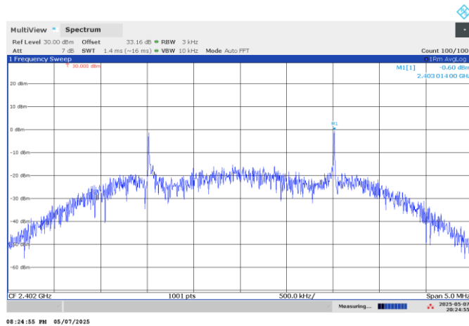
Figure 7.7-1: PSD on low channel
