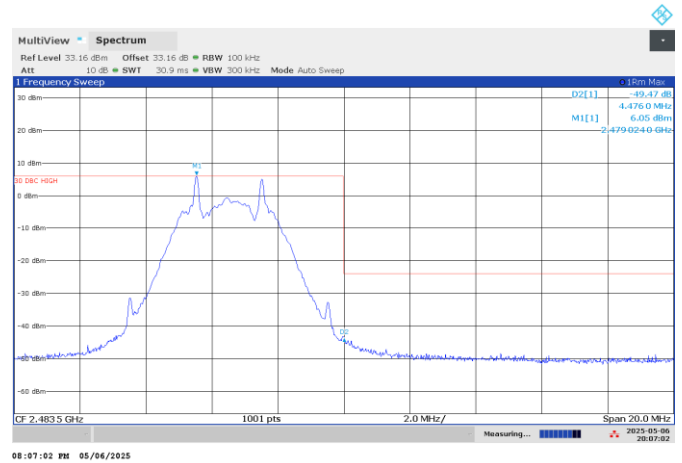
Figure 7.6-2: Band edge spurious emissions at 2483.5 MHz
