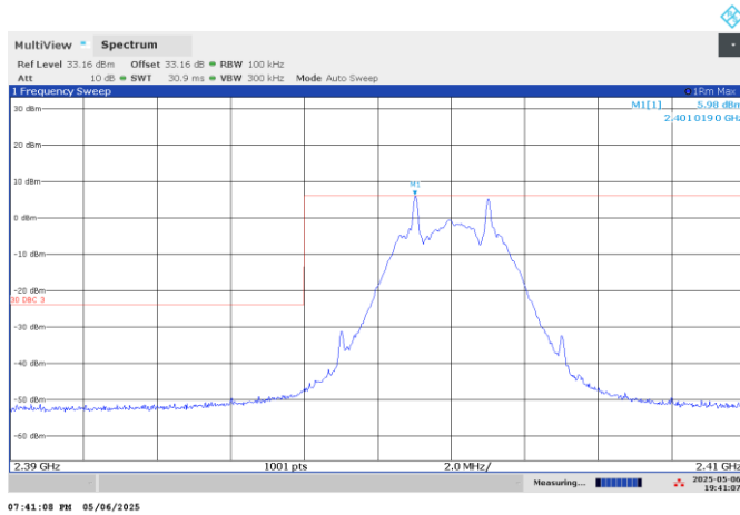
Figure 7.6-1: Band edge spurious emissions at 2400 MHz
