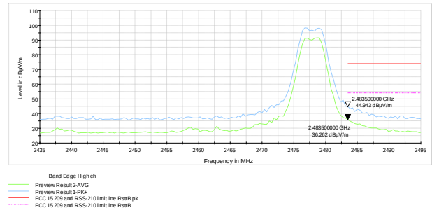
Figure 7.6-4: Band edge spurious emissions at 2483.5 MHz
