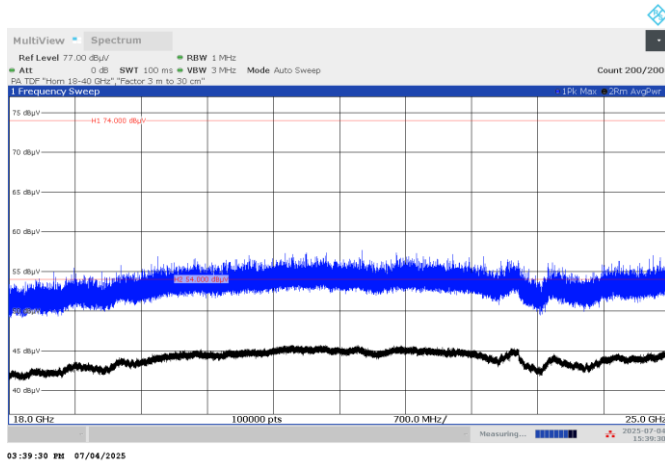
Figure 7.6-17: Radiated spurious emissions on 18 -25 GHz, Low ch.
