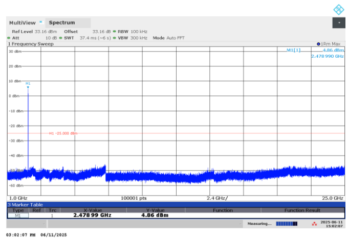
Figure 7.6-10: Radiated spurious emissions on above 1 GHz, High ch.
