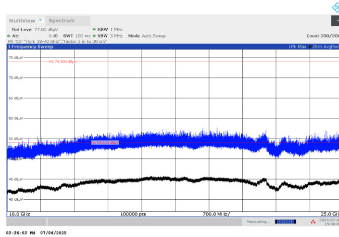
Figure 7.6-19: Radiated spurious emissions on 18 -25 GHz, High ch.
