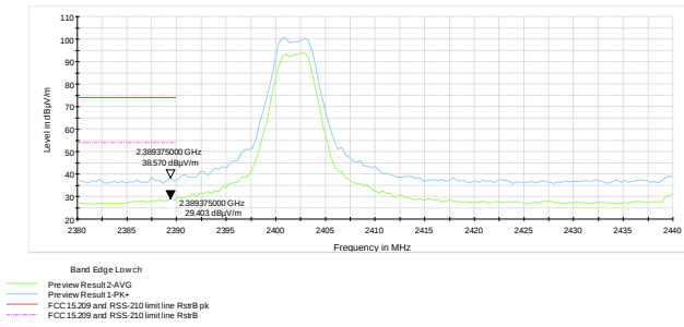
Figure 7.6-3: Band edge spurious emissions at 2390 MHz
