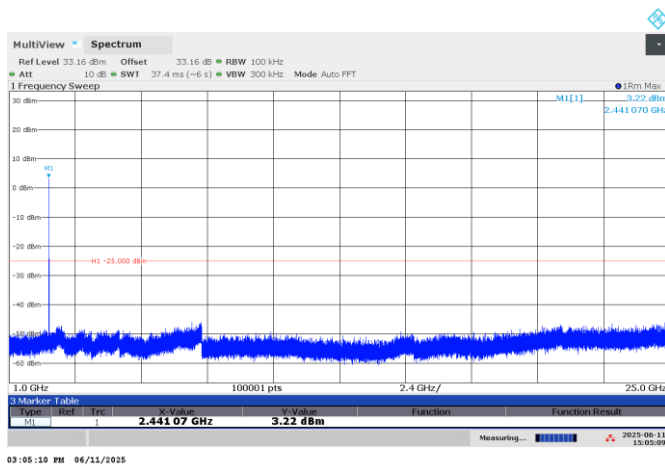
Figure 7.6-9: Radiated spurious emissions on above 1 GHz, Mid ch.
