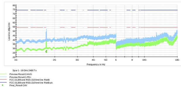
Figure 7.6-16: Radiated spurious emissions on 1 - 18 GHz, High ch.
