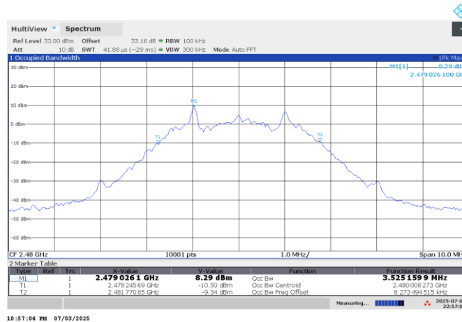
Figure 7.4-6: 99% occupied bandwidth on GFSK, High ch
