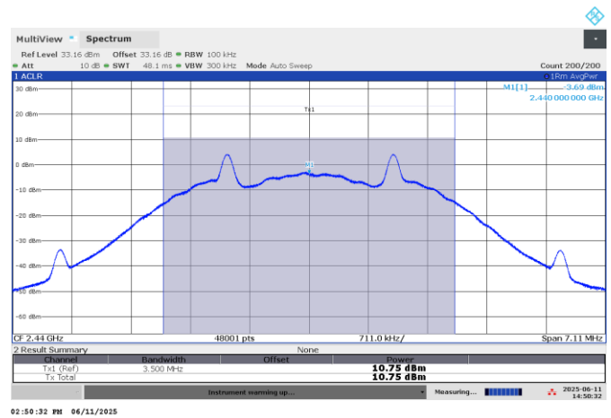
Figure 7.5-2: Output power on mid channel
