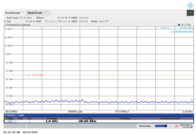
Figure 7.6-6: Conducted spurious emissions on below 1 GHz, Mid ch.
