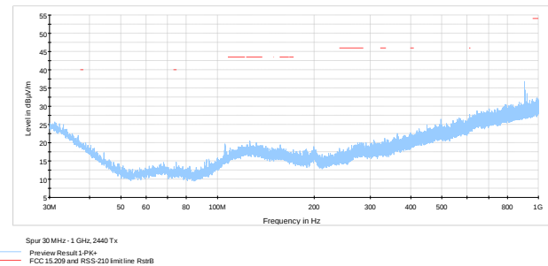
Figure 7.6-12: Radiated spurious emissions on below 1 GHz, Mid ch.
