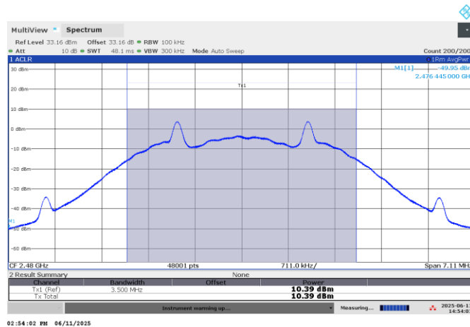
Figure 7.5-3: Output power on high channel
