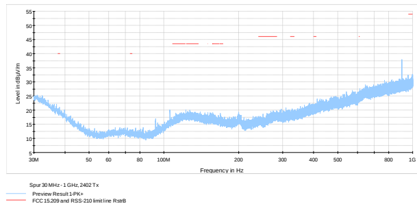
Figure 7.6-11: Radiated spurious emissions on below 1 GHz, Low ch.
