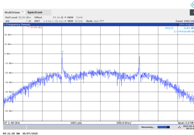
Figure 7.7-3: PSD on high channel
