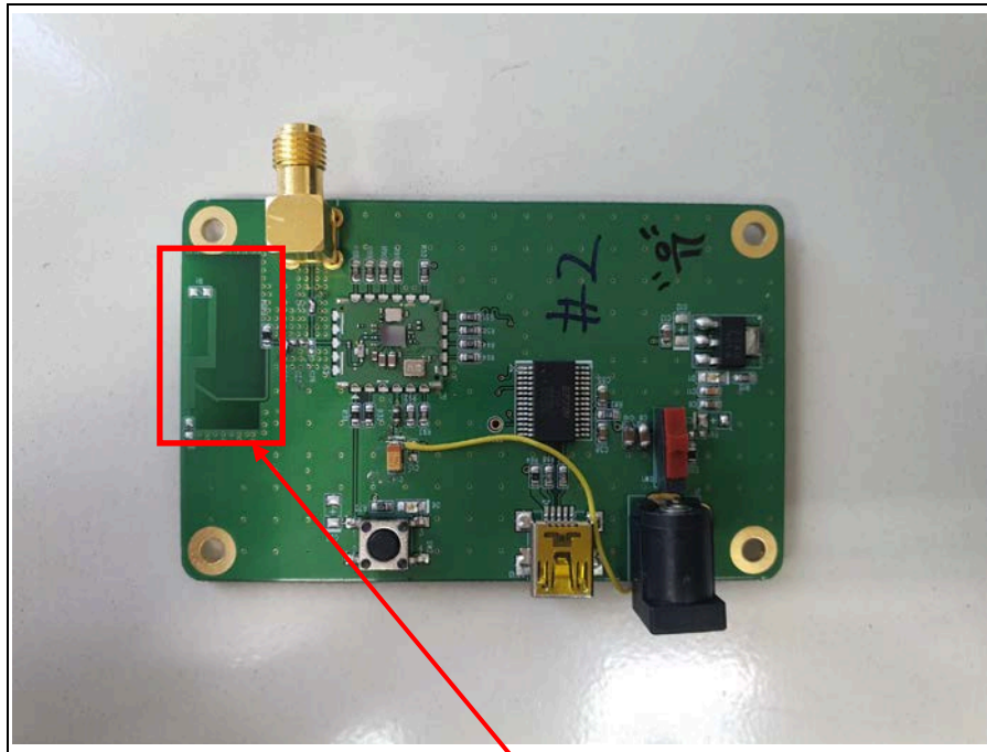
BT Antenna
