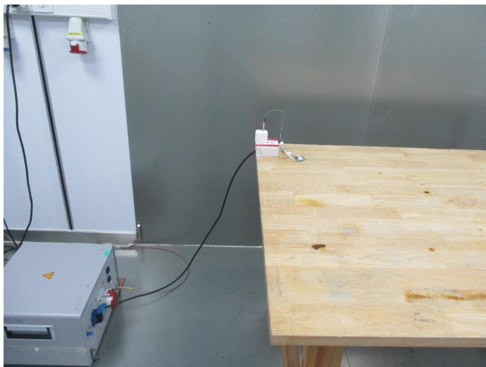
Conducted Emission
