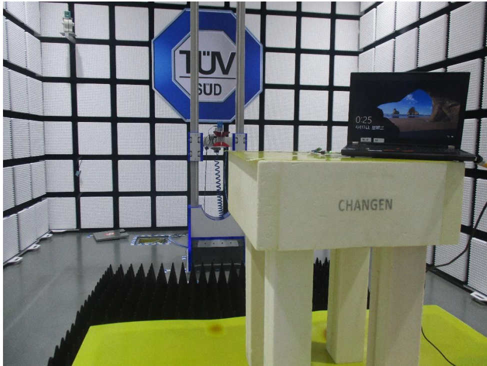
Radiated Emission Test below 1GHz-18GHz
