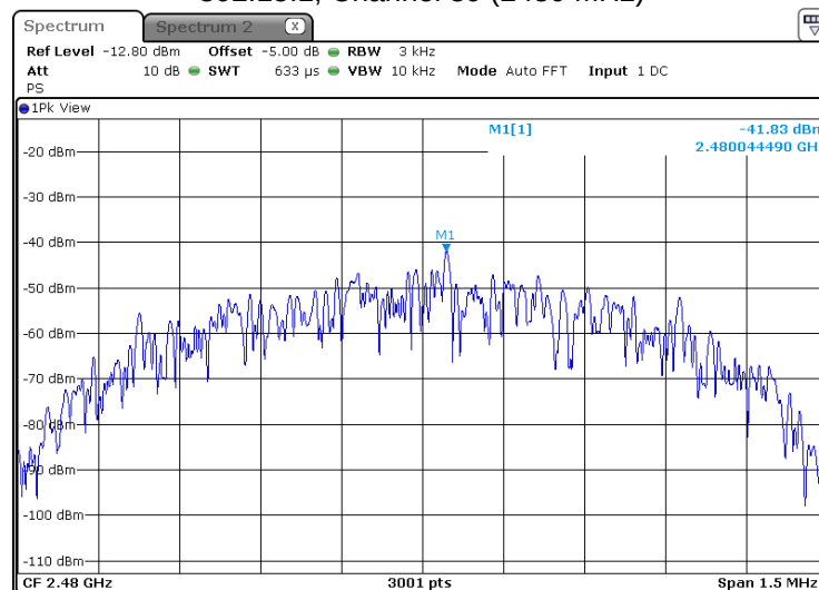
802.15.1, Channel 39 (2480 MHz)
