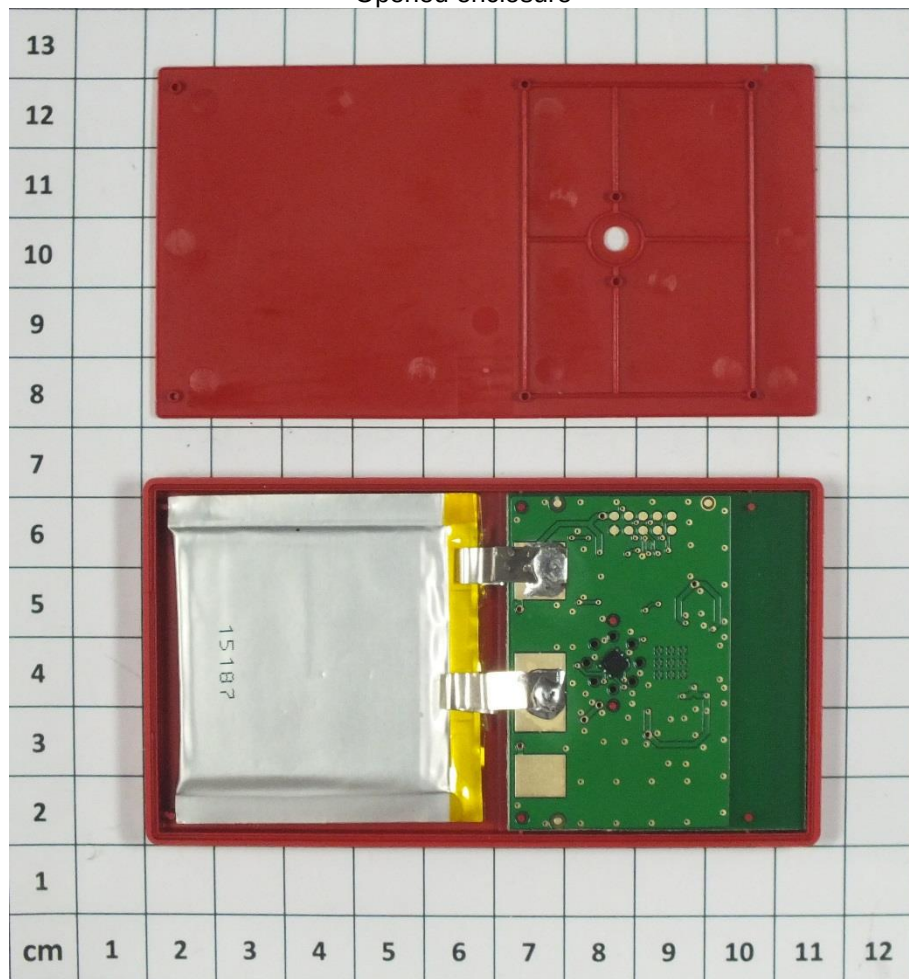
Opened enclosure
